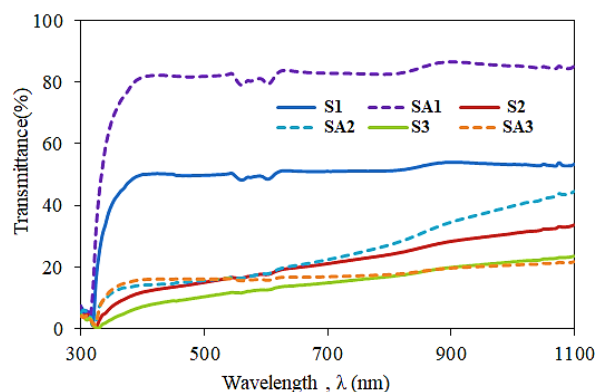
Fig. 14. Transmittance spectra as a function of photon wavelength for the considered samples
